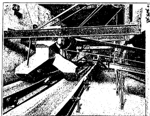
Weller Belt Conveyors and Trippers in Large Grain Elevator.
